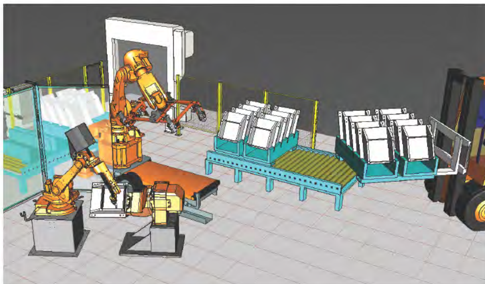
Arc welding simulation with RobotExpert.
