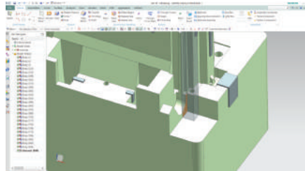
Auto Interference check between Electrode Head and Steel Insert
