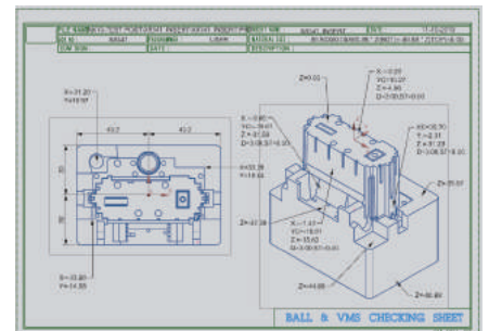
Auto Electrode / Steel Insert QC Check Sheet
