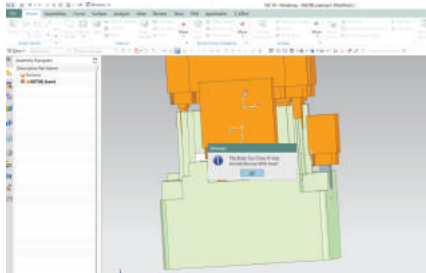
Auto Electrode Body Extension to Avoid Collision between Electrode Holder and Steel Insert
